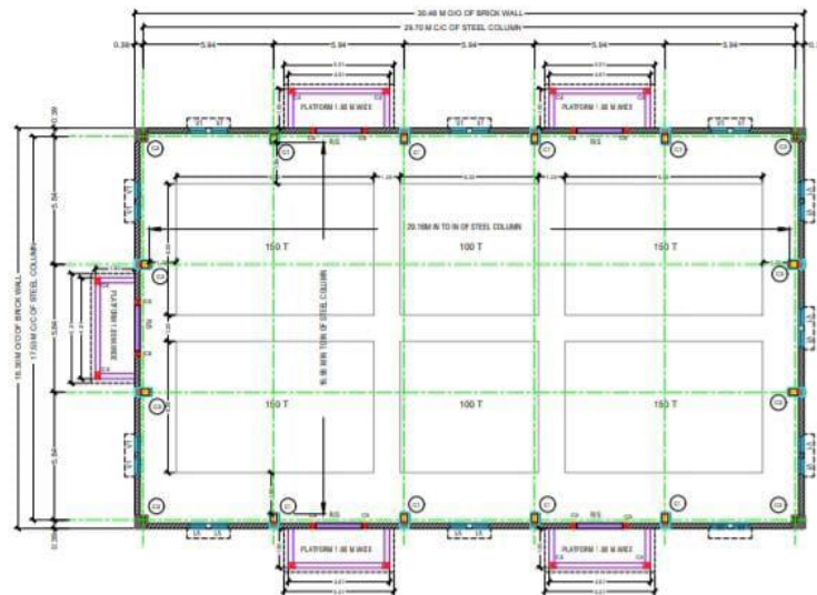
PLAN FOR 800 MT UNIT
