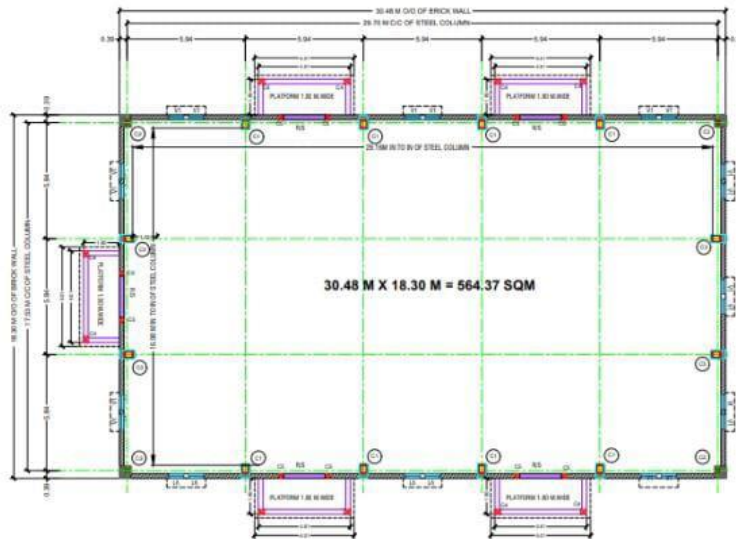
INDUSTRIAL SHED PLAN
