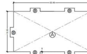
BLOCK PLAN
